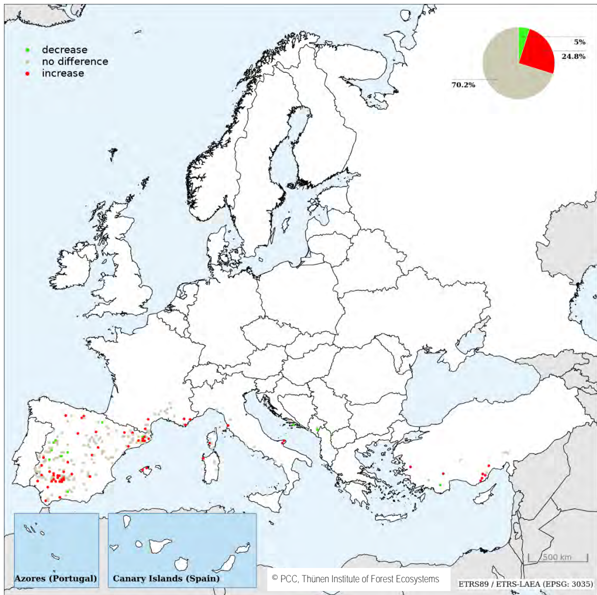
Figure S1-16: Trends in mean plot defoliation of evergreen oaks ( Quercus coccifera , Q ilex , Q. rotundifolia , Q. suber ) between 2013 and 2022. Plots were included if assessments were available for at least 80% of the period. The legend (top left) indicates whether mean plot defoliation overall decreased, stayed the same or increased within the given period. The pie chart (top right) indicates the respective percentage of plots per trend direction.
