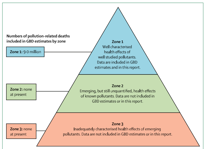
Figure 3: The pollutome
