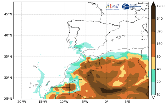
Barcelona Dust Forecast Center - http://dust.aemet.es/ NMMB-MONARCH Res:0.1°x0.1° Dust Surface Conc. ( \mu\text{g}/\text{m}^3 ) Run: 12h 05 APR 2021 Valid: 12h 07 APR 2021 (H+48)
