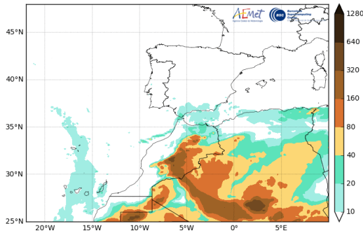
Barcelona Dust Forecast Center - http://dust.aemet.es/ NMMB-MONARCH Res:0.1°x0.1° Dust Surface Conc. ( \mu\text{g}/\text{m}^3 ) Run: 12h 05 APR 2021 Valid: 00h 07 APR 2021 (H+36)
