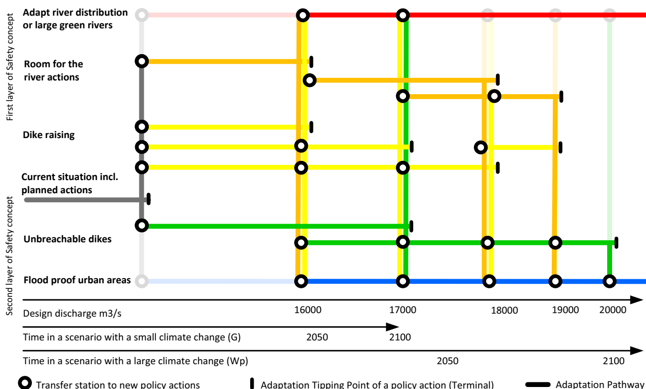
Figure 5.2 Adaptation pathway map for the River Waal
