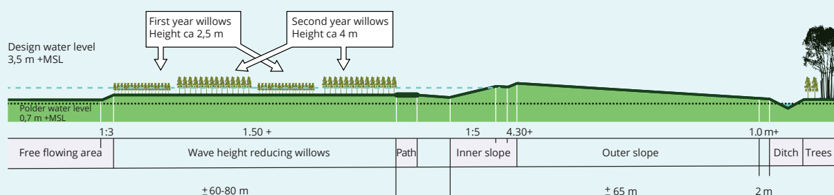
Figure 5.1 Schematics of Nature- based flood protection in the Noordwaard (The Netherlands)
