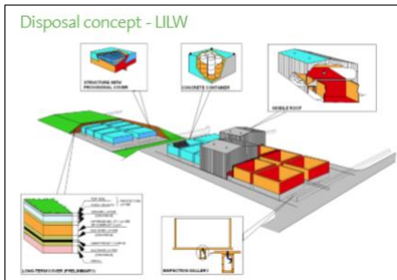
Figure 5: El Cabril disposal concept.
