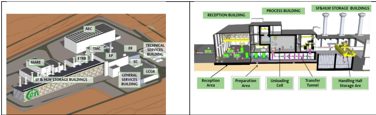
Figure 6: Centralized storage facility (CSF) and cross section of the main process building.
